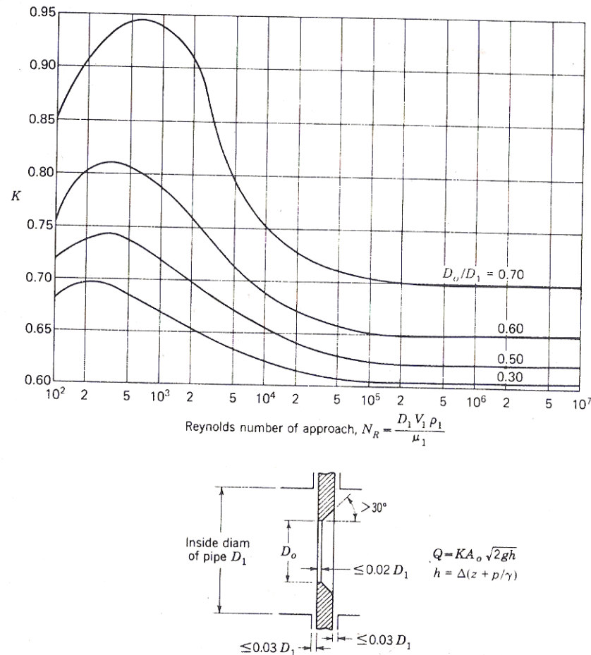
Figure 12.23. VDI orifice meter and flow coefficients for flange taps. (Adapted from NACA Tech. Mem. 952 .)
